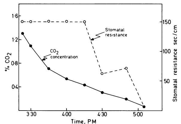
FIG. 2. Kinetics of decline in internal gas phase CO 2 concentration and stomatal resistance to diffusion of water vapor at the end of the day in O. ficus-indica .
